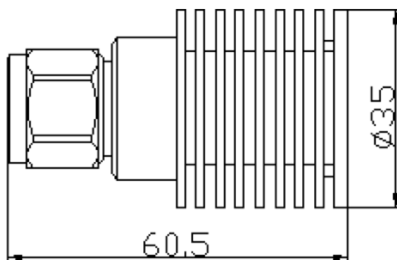
TE-10W-6GNM (Round type)
