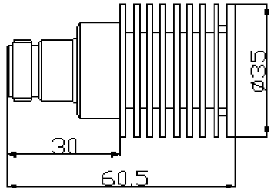
TE-10W-6GNF (Round type)
